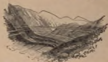
FIG. 349.—The "parallel roads" of Glen Roy in the southern highlands of Scotland (after Jamieson).
